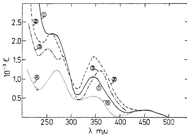
Figure 1.—Spectra of Cr(VI) species ( \epsilon is molar absorptance): 1, solid line, \text{CrSO}_4^{2-} , measured directly; 2, dashed line, \text{HCrO}_4^- , measured directly; 3, dash-dot line, \text{CrO}_5\text{Cl}^- , measured directly; 4 dotted line, \text{H}_2\text{CrO}_4 , calculated from mixed spectrum and K_D .
